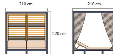
Cabana - double lounger with pergola 210x210x220 cm Index: 804302571 Weight: 150 kg
