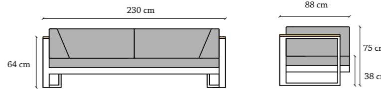
Sofa Toscana 2-person 230x88x75 cm Index: 191008 Weight: 30 kg
