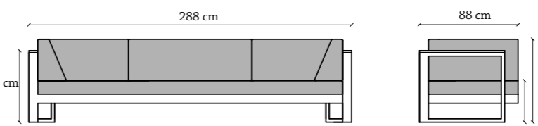
Sofa Toscana 3-person 288x88x75 cm Index: 191002 Weight: 38 kg
