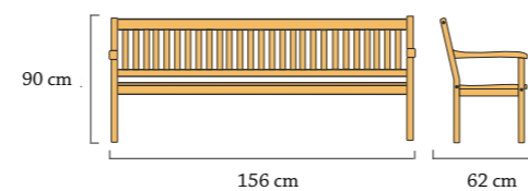
Bench Kansas 3-person 156×62×90 cm Index: 010104 Weight: 29 kg
