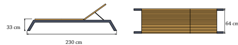
Lounger Ripper 230x64x33 cm Index: 025302571 Weight: 30 kg
