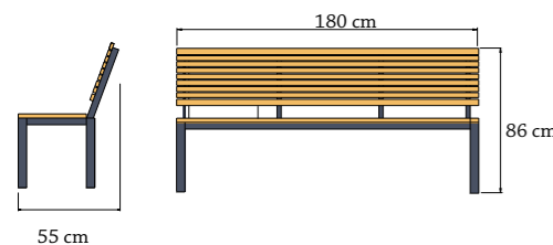
Bench Ripper 180 180x55x86 cm Index: 021302571 Weight: 28 kg
