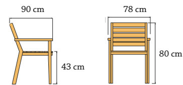
Armchair Caro 78x90x80 cm Index: 001000571 Weight: 10 kg
