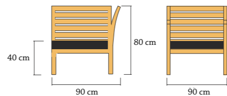
Corner Milano 90x90x80 cm Index: 190110 Weight: 19,6 kg
