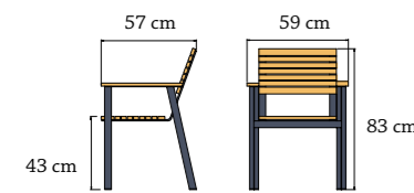
Armchair Ripper 60x57x83 cm Index: 020302571 Weight: 9 kg
