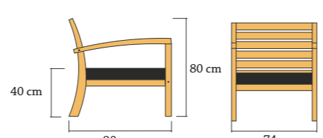
Armchair Milano with right arm 74x90x80 cm Index: 190108 Weight: 13 kg
