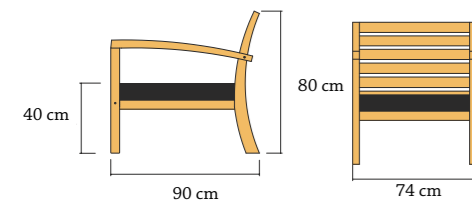
Armchair Milano with left arm 74x90x80 cm Index: 190109 Weight: 13 kg
