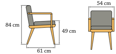
Armchair Bouhus 54x61x84 cm Index: 80604571 Weight: 12 kg
